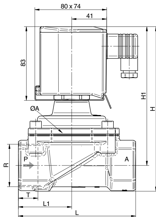
DN 32 - DN 50
